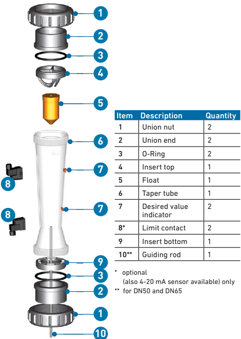
Fig. 1: Variable area flow meter
